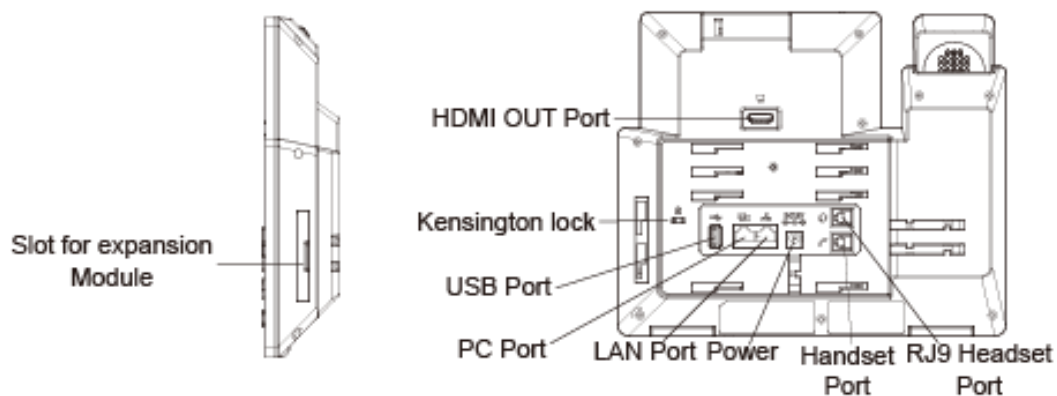
Figure 6: GXV3350 Back / Side View
