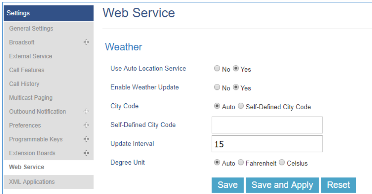
Figure 9: Web Service
